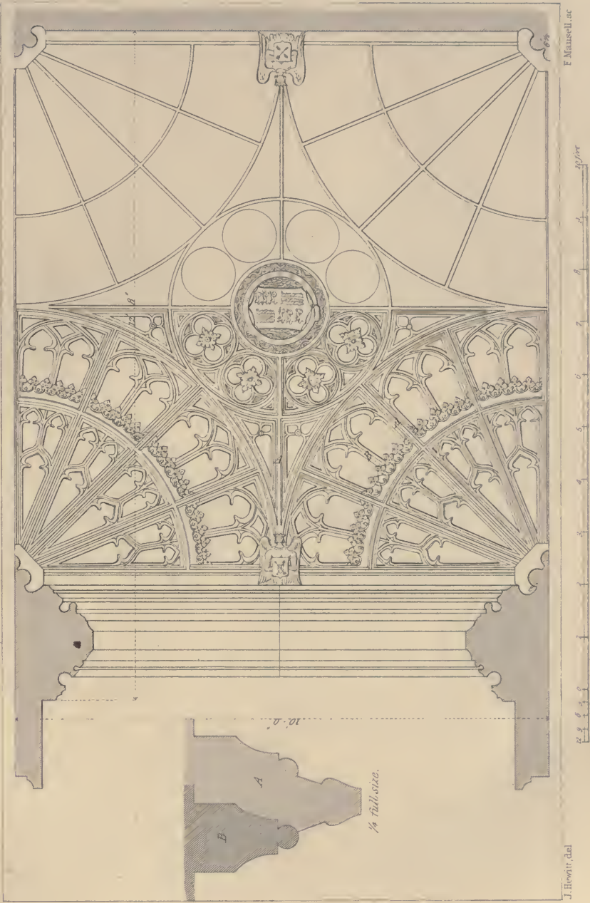
COMPARTMENT OF CEILING AT NORTH AND SOUTH SIDES.
